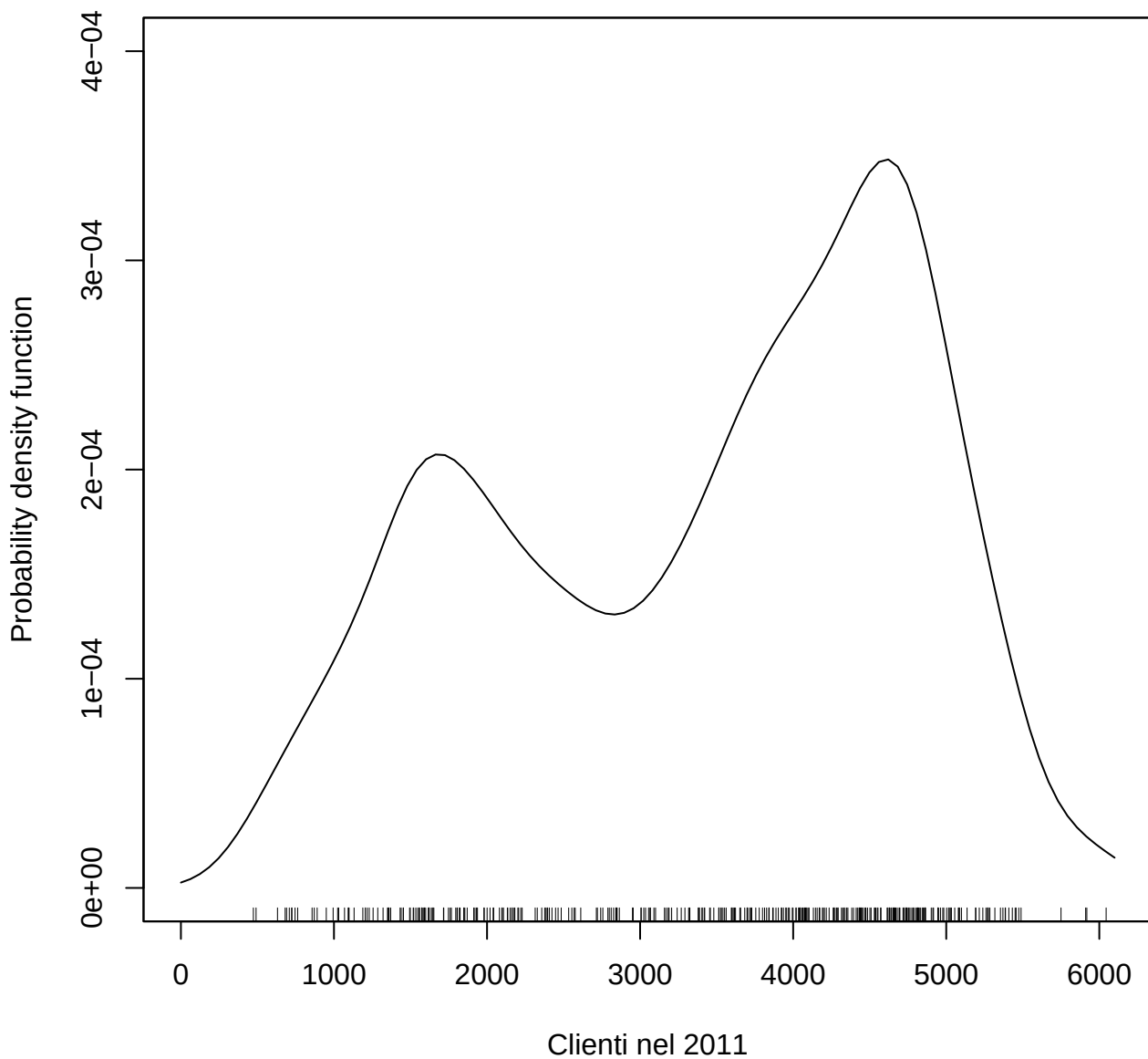
Kernel density estimation ('CV' h = 252.063)
